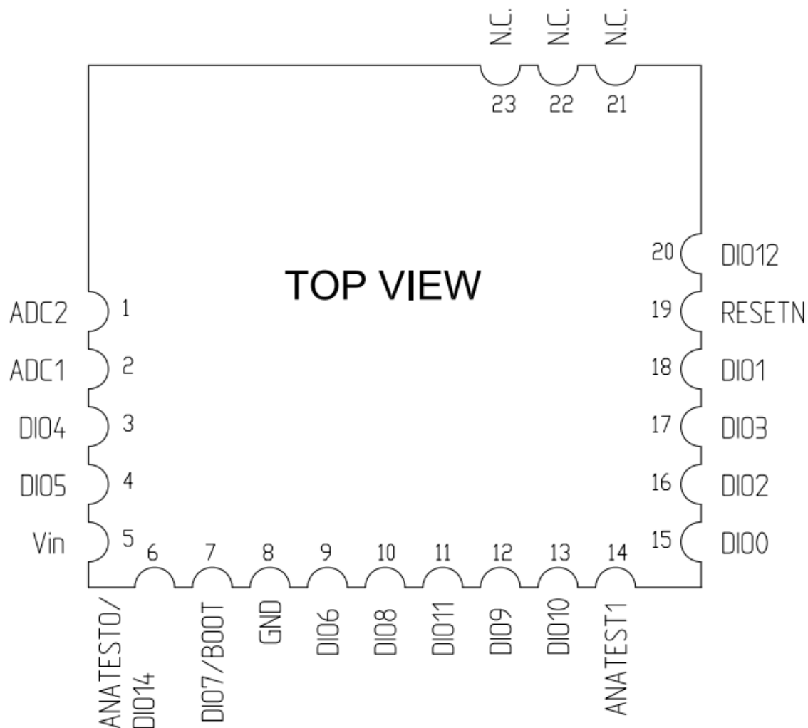
Figure 7: Pin assignment
