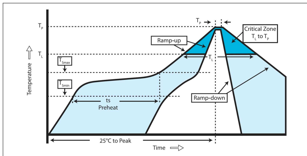
Figure 11: Soldering profiles
