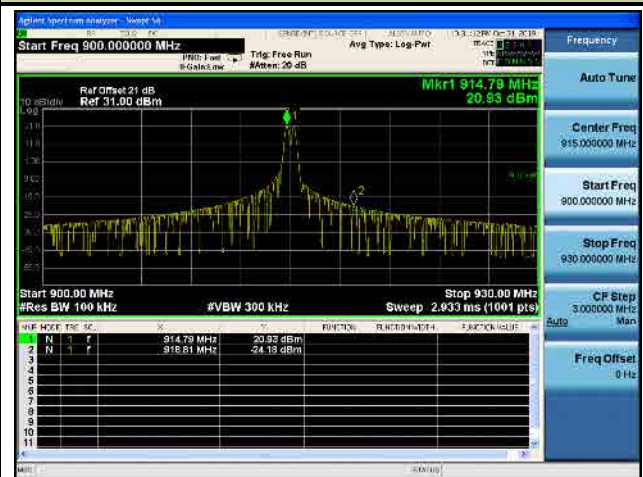
2FSK-915MHz
