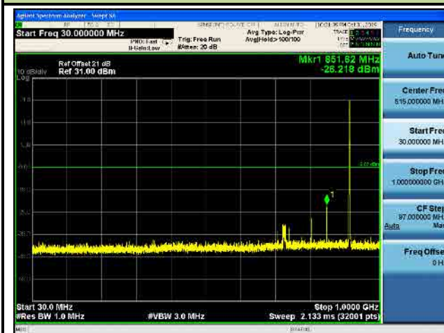
2FSK-915MHz
