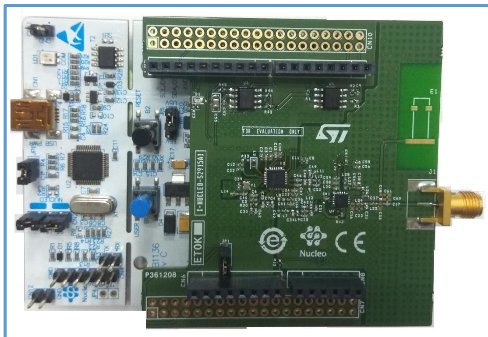
Figure 2. X-NUCLEO-S2915A1 expansion board connected to an STM32 Nucleo development board
