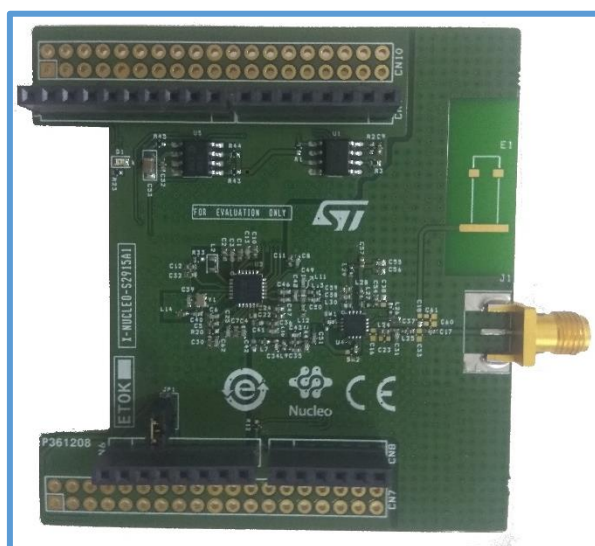
Figure 1. Sub-1 GHz expansion board based on S2-LP for STM32
