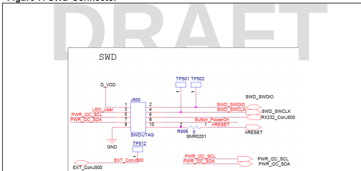
Figure 7: SWD Connector
