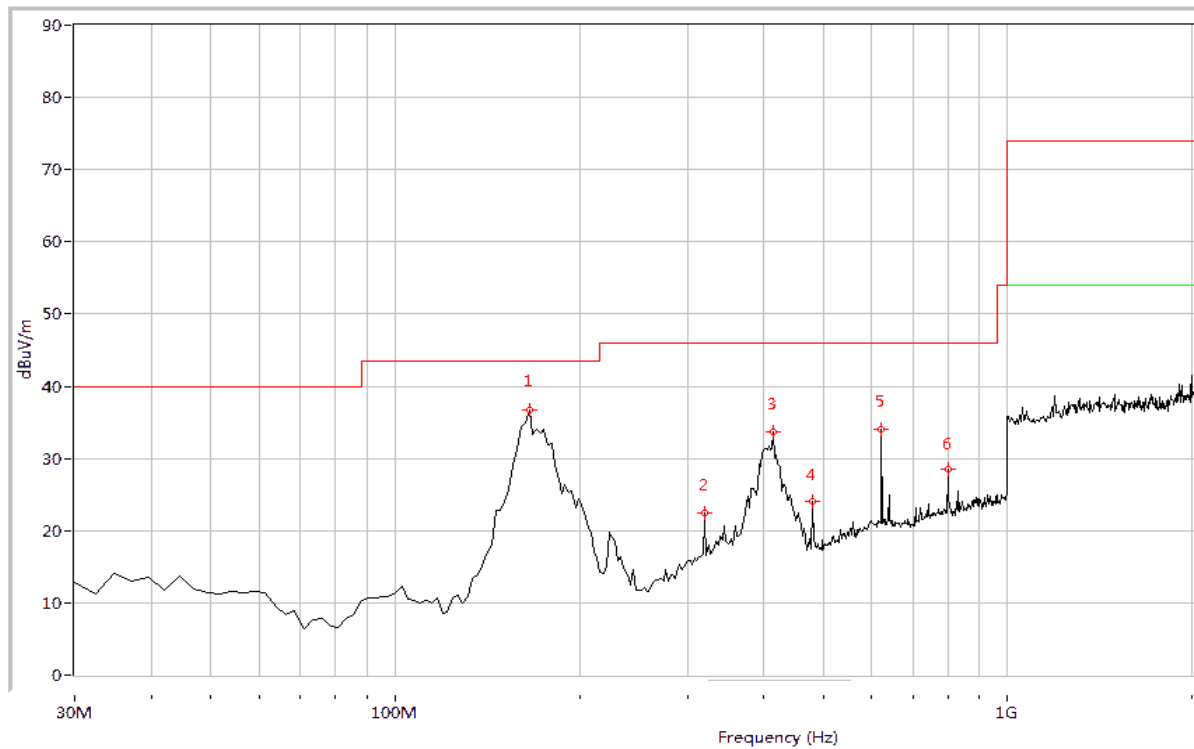
(Plot C: 30MHz – 2GHz, Test Antenna Horizontal)
