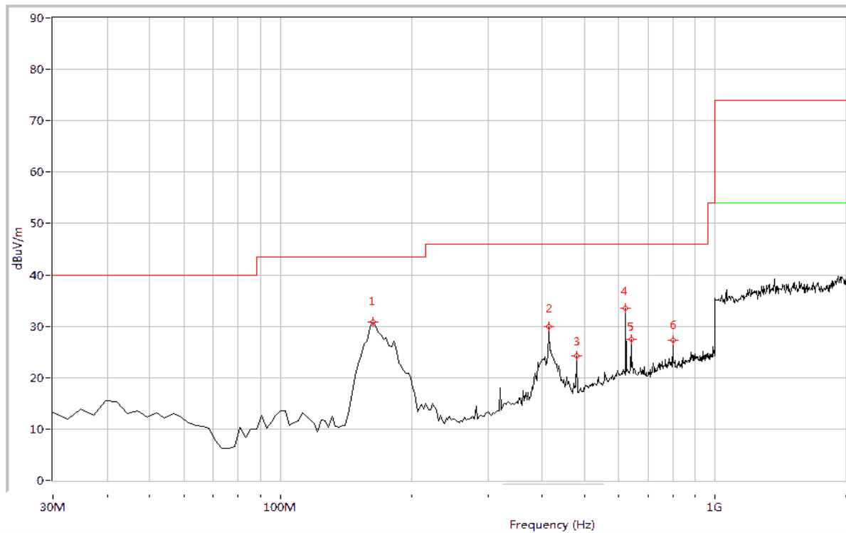
(Plot B: 30MHz – 2GHz, Test Antenna Vertical)
