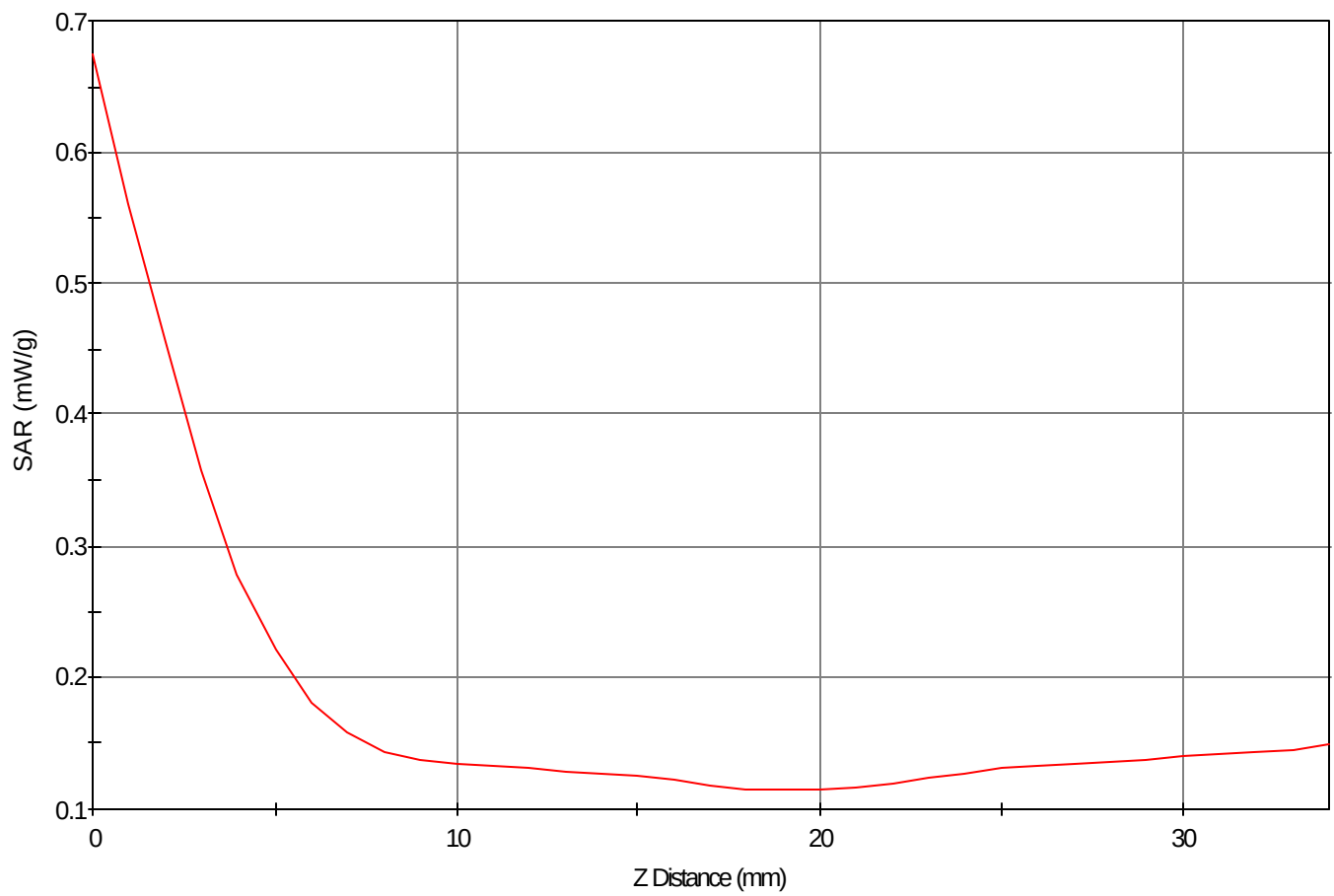
SAR - Z Axis at Hotspot x:-1.0 y:12.0
