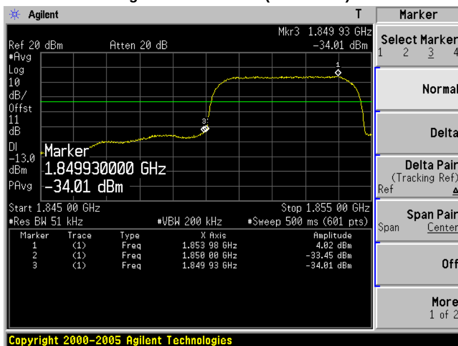
Figure Channel 9262 (1852.4MHz)
