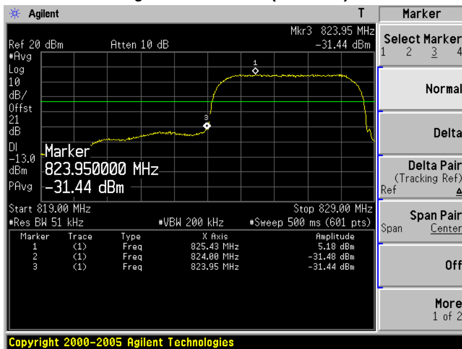
Figure Channel 4132 (826.4MHz)
