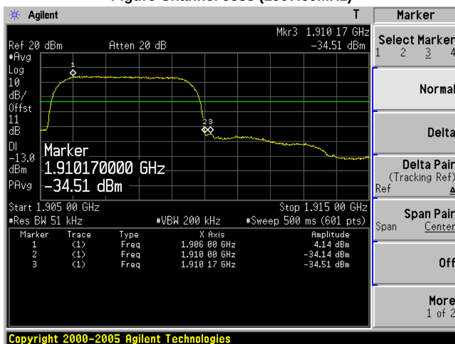
Figure Channel 9538 (1907.60MHz)
