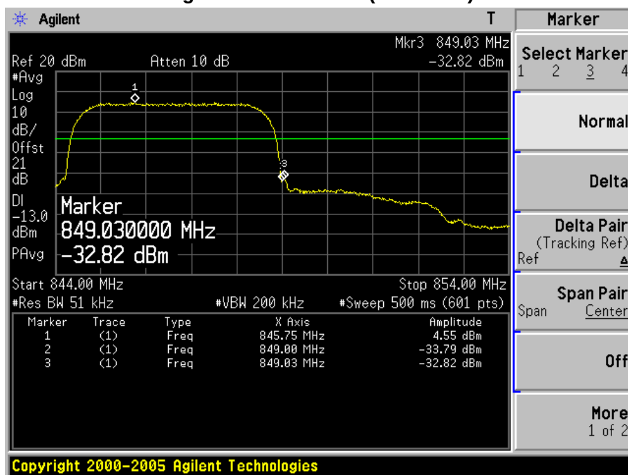
Figure Channel 4233 (846.6MHz)
