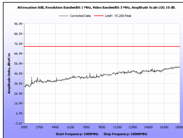
Plot 15. Radiated Spurious Emissions, 802.11b, 2462 MHz, 1 GHz – 18 GHz, Peak
