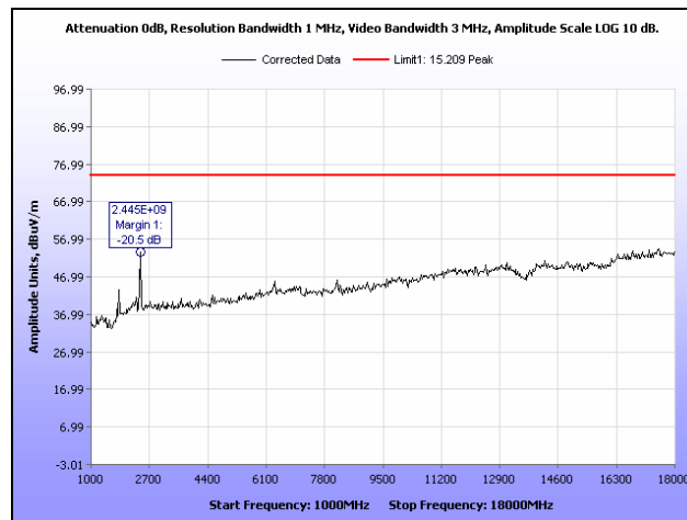
Plot 12. Radiated Spurious Emissions, 802.11b, 2437 MHz, 1 GHz – 18 GHz, Peak
