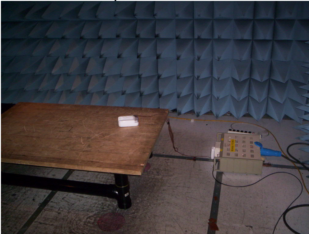
Spurious Emissions Setup:
