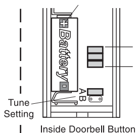
Inside Doorbell Button
