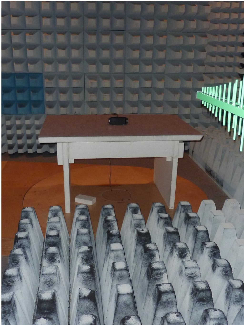
150998_d.JPG: OptiTire ECU, test set-up fully anechoic chamber
