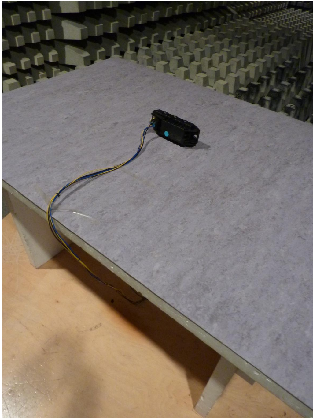
150998_a.JPG: OptiTire ECU, test set-up fully anechoic chamber, pos. 2
