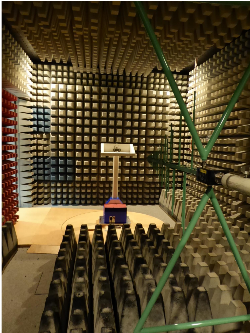
162386_21.JPG: WM2.4, test set-up fully anechoic chamber
