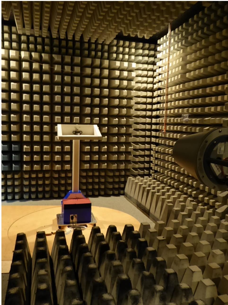
162386_22.JPG: WM2.4, test set-up fully anechoic chamber
