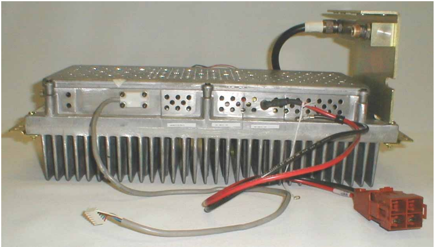
External View of MASTR III Power Amplifier
