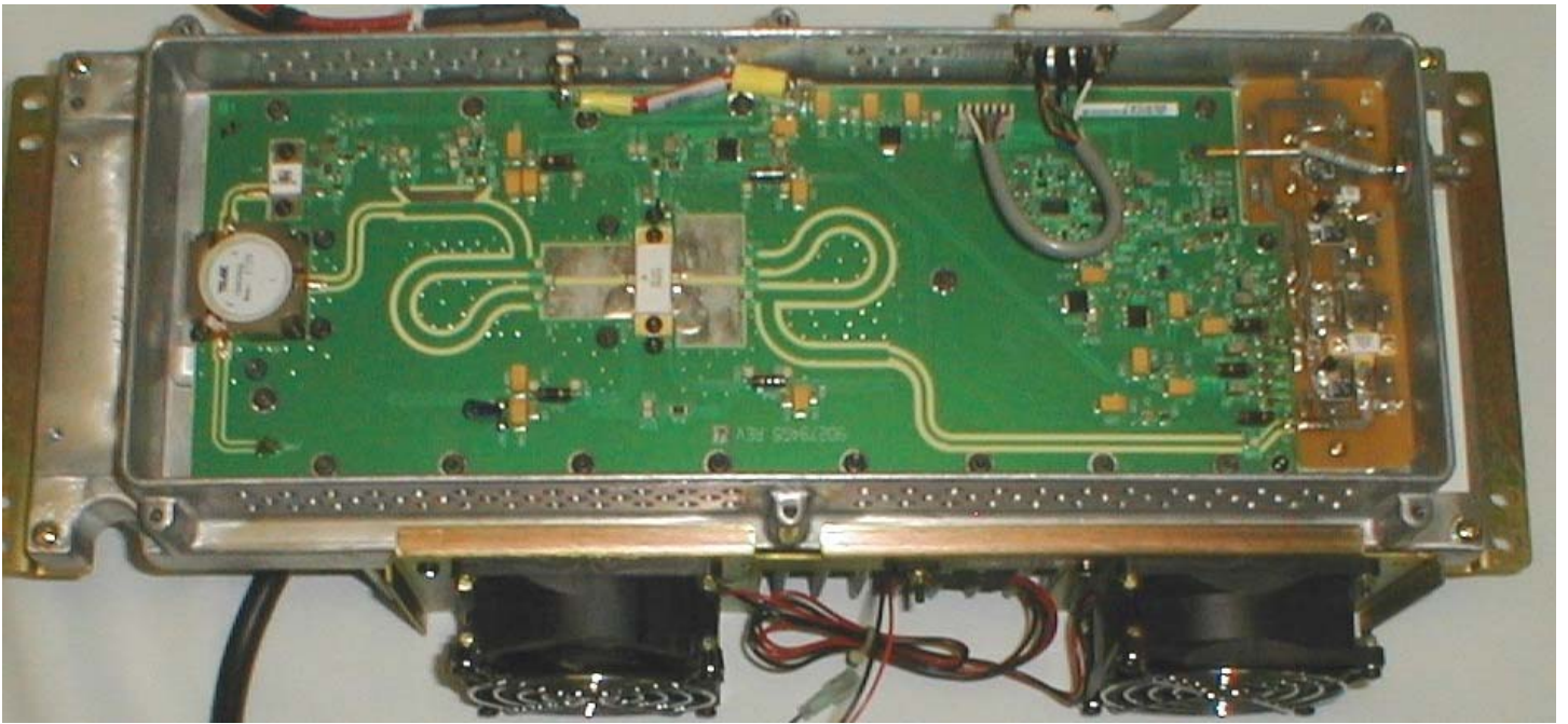
19D902797G Power Amplifier Board
