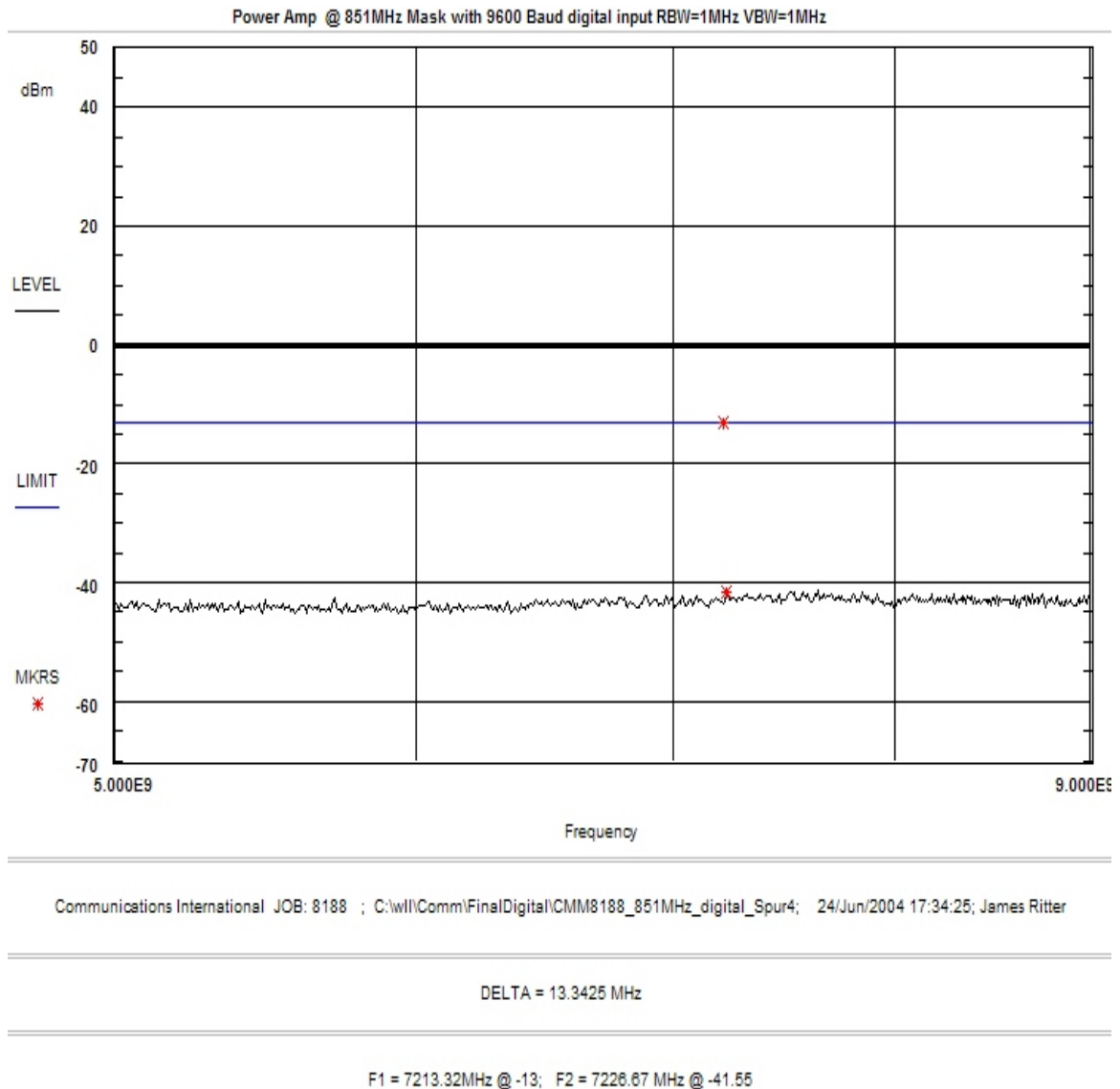
Figure 16. Conducted Spurious Emissions, 851 MHz Digital Modulation F1D, F1E, F2D, F2B
