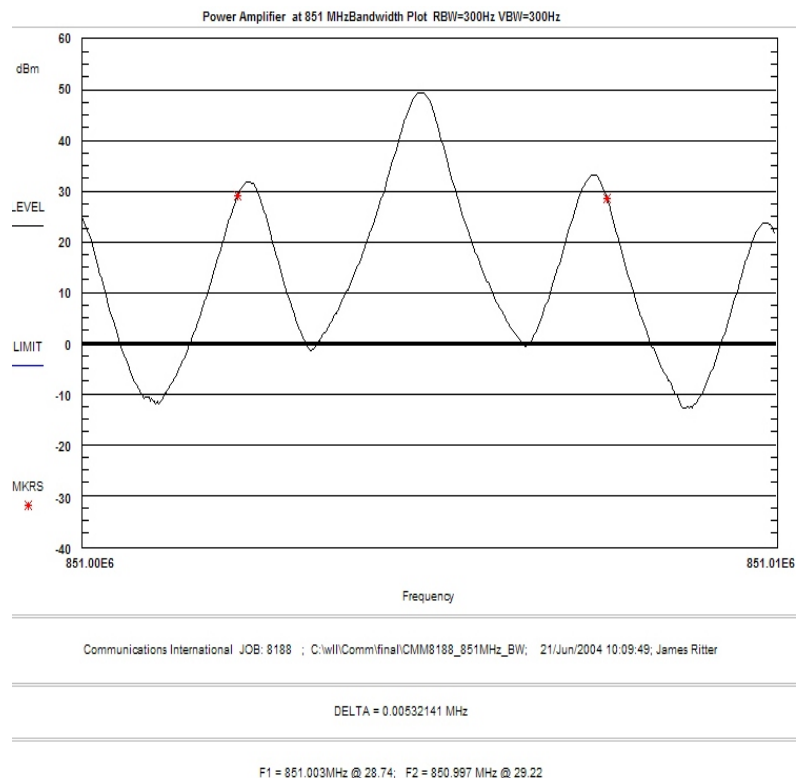
Figure 1. Occupied Bandwidth: 851 MHz Analog Modulation, F3E
