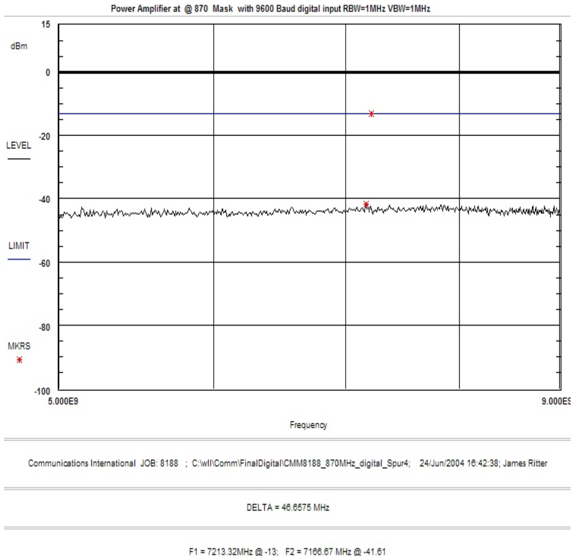
Figure 34. Conducted Spurious Emissions, 870 MHz Digital Modulation F1D, F1E, F2D, F2B
