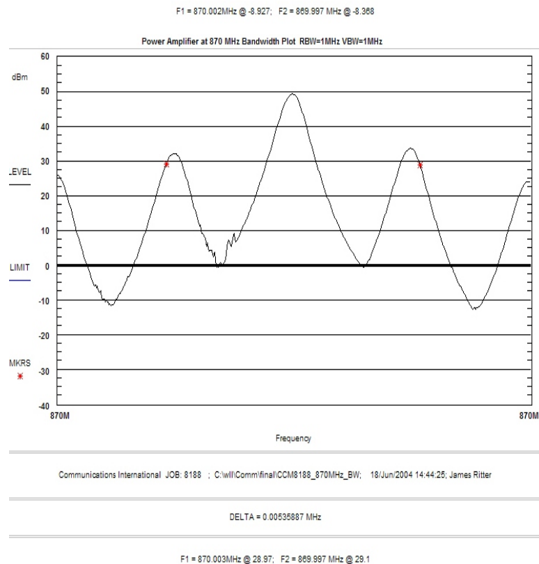
Figure 5. Occupied Bandwidth 870 MHz Analog Modulation, F3E
