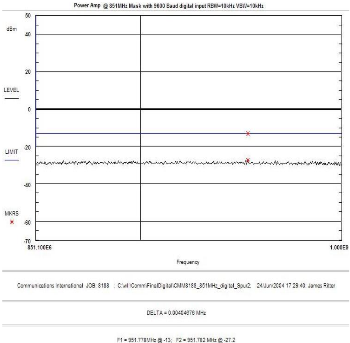
Figure 14. Conducted Spurious Emissions, 851 MHz Digital Modulation F1D, F1E, F2D, F2B
