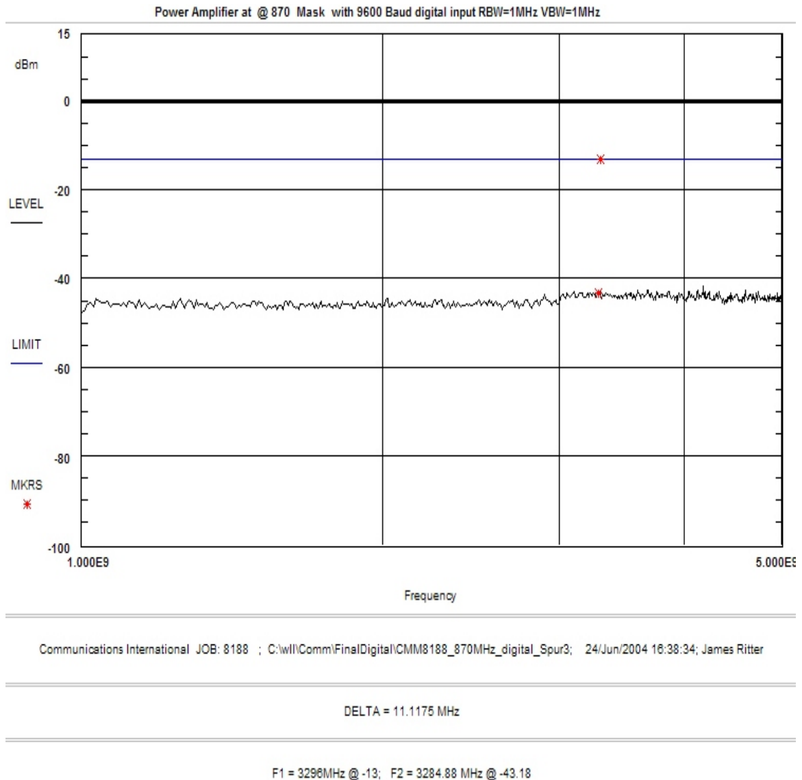
Figure 33. Conducted Spurious Emissions, 870 MHz Digital Modulation F1D, F1E, F2D, F2B
