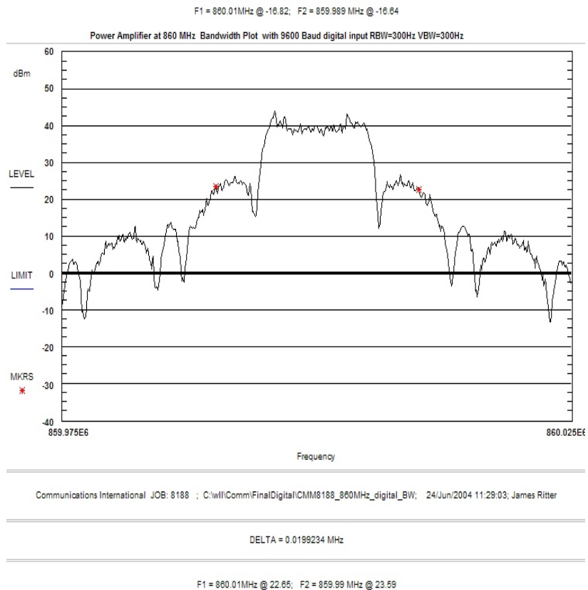
Figure 4. Occupied Bandwidth 860 MHz Digital Modulation F1D, F1E, F2D, F2B
