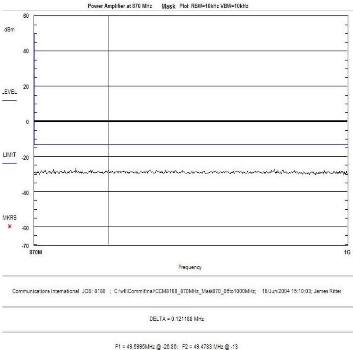
Figure 28. Conducted Spurious Emissions, 870 MHz Analog Modulation, F3E
