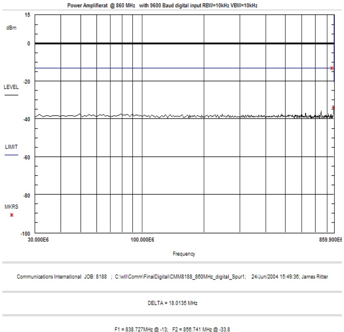
Figure 23. Conducted Spurious Emissions, 860 MHz Digital Modulation F1D, F1E, F2D, F2B
