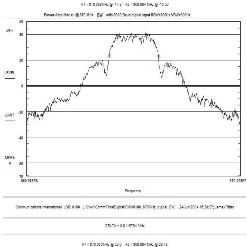
Figure 6. Occupied Bandwidth 870 MHz Digital Modulation F1D, F1E, F2D, F2B
