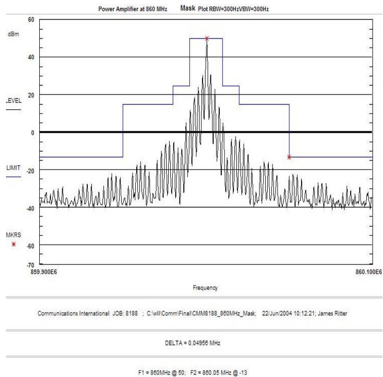
Figure 17. Mask, 860 MHz Analog Modulation, F3E
