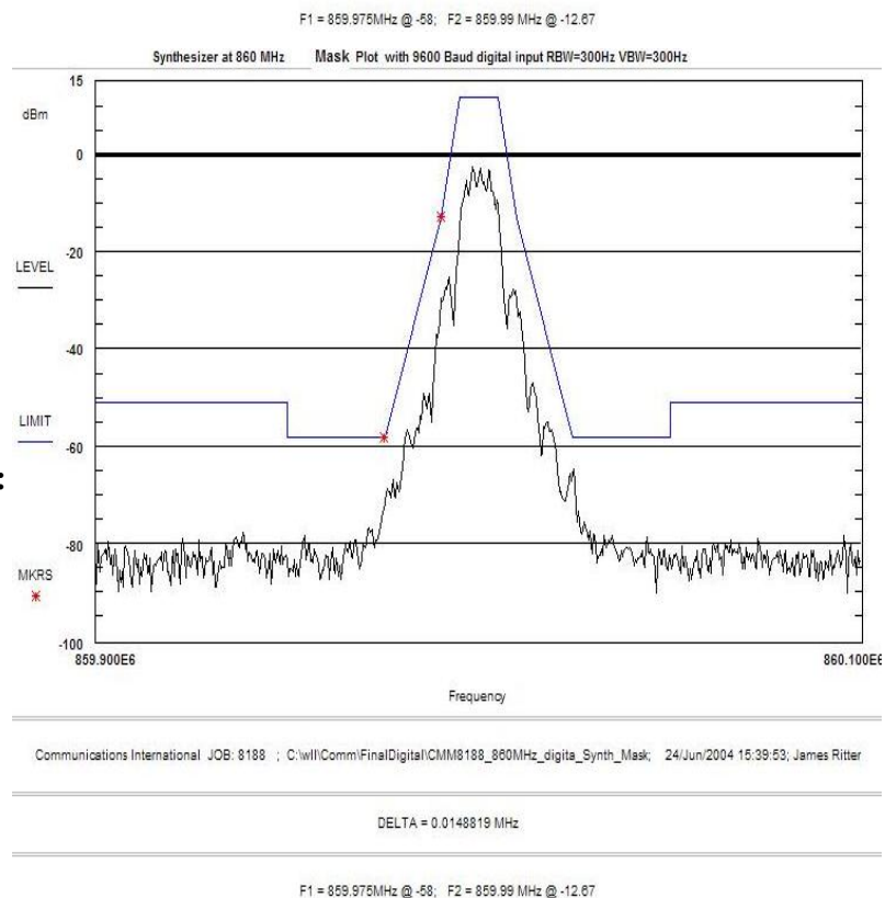
Figure 22. Mask, 860 MHz Digital Modulation F1D, F1E, F2D, F2B
