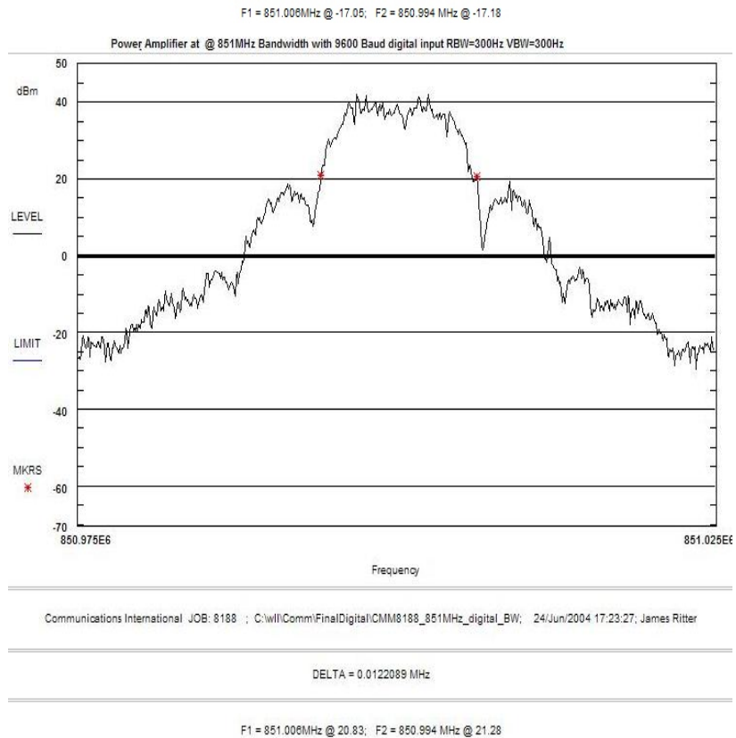
Figure 2. Occupied Bandwidth 851 MHz Digital Modulation, F1D, F1E, F2D, F2B
