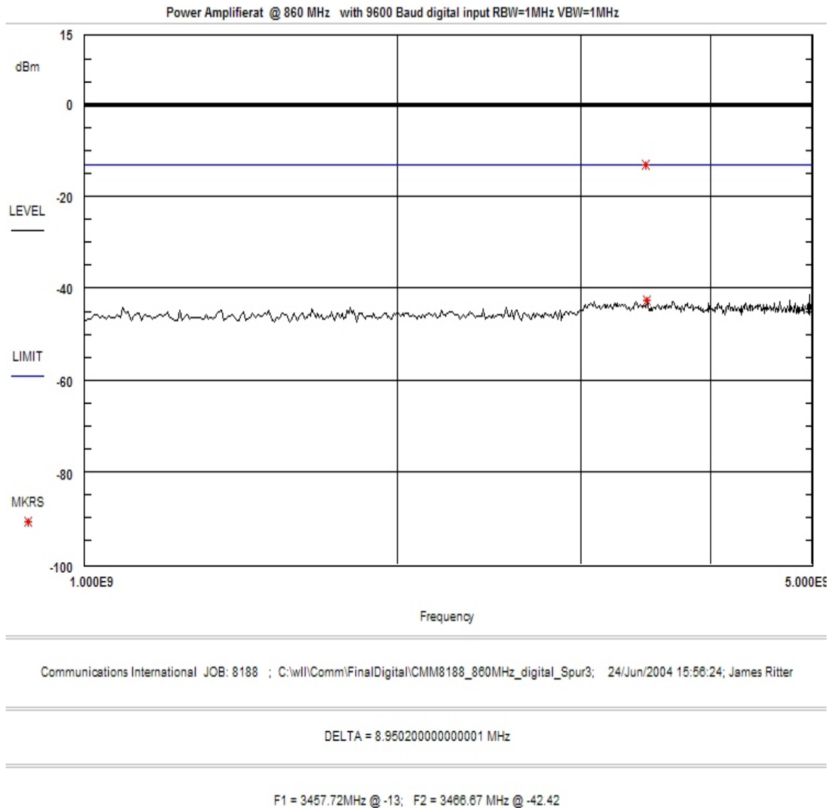
Figure 24. Conducted Spurious Emissions, 860 MHz Digital Modulation F1D, F1E, F2D, F2B
