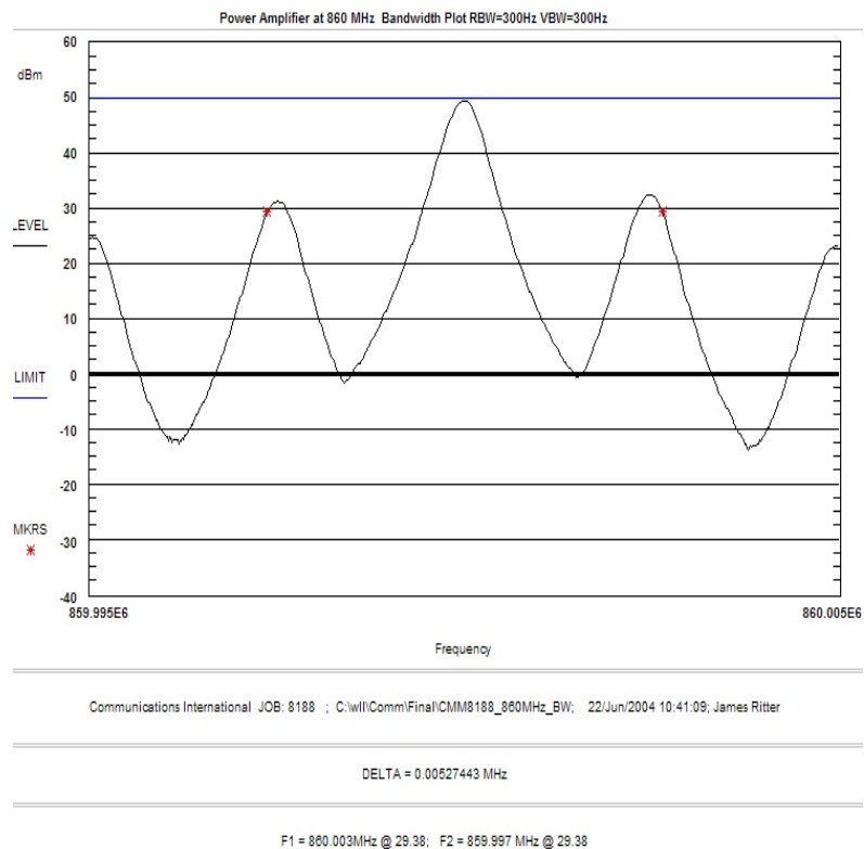
Figure 3. Occupied Bandwidth 860 MHz Analog Modulation, F3E
