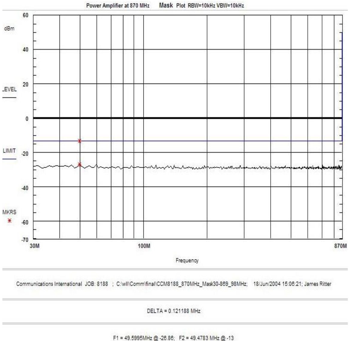
Figure 27. Conducted Spurious Emissions, 870 MHz Analog Modulation,F3E
