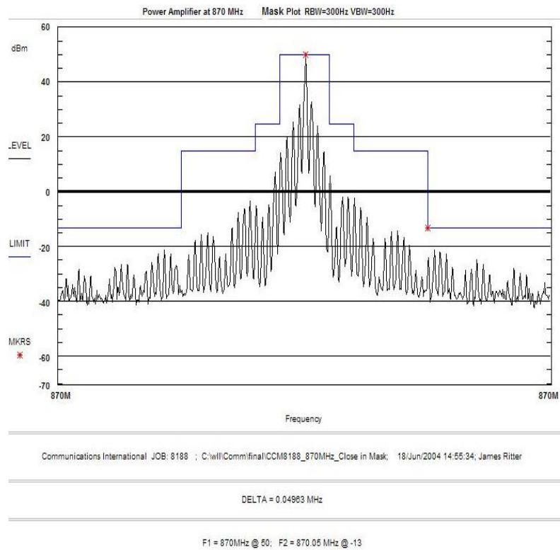
Figure 26. Mask, 870 MHz Analog Modulation, F3E
