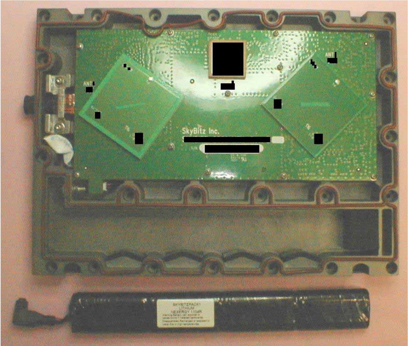
Battery Removed
