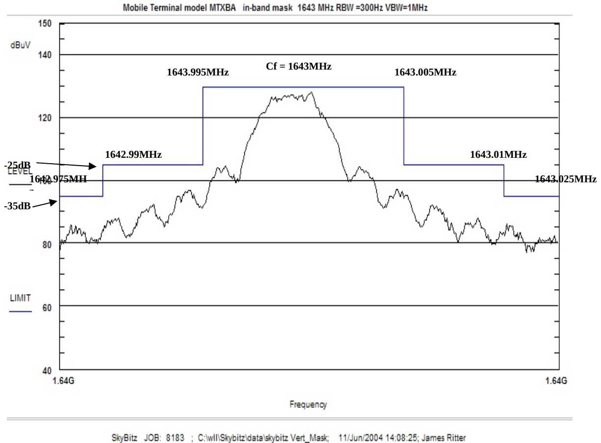
Figure 3: Emission Mask, Vertical
