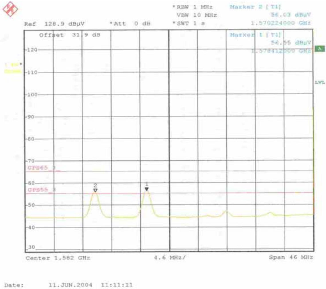
Figure 4: Spurious Emissions 1559M – 1605MHz, Vertical Polarity
