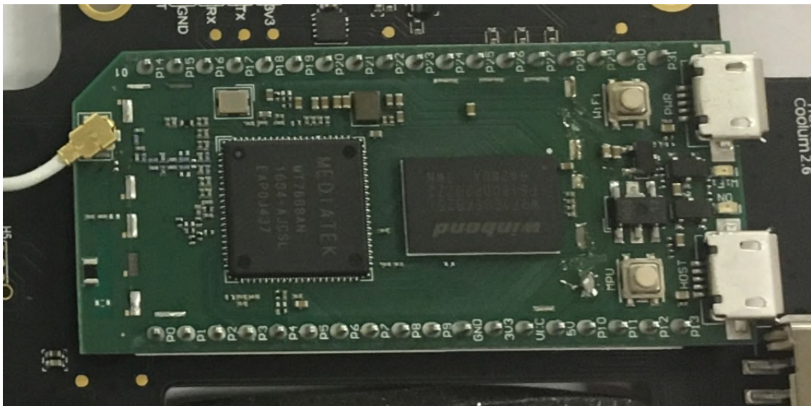
Figure 3: Module – Front
