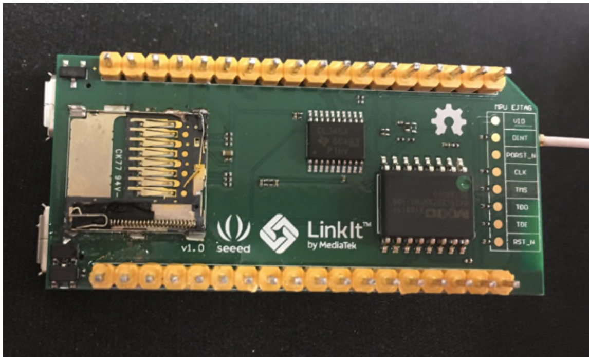
Figure 7: Module without Shields - Back
