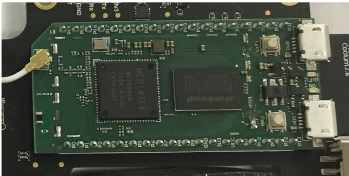
Figure 3: Module – Front
