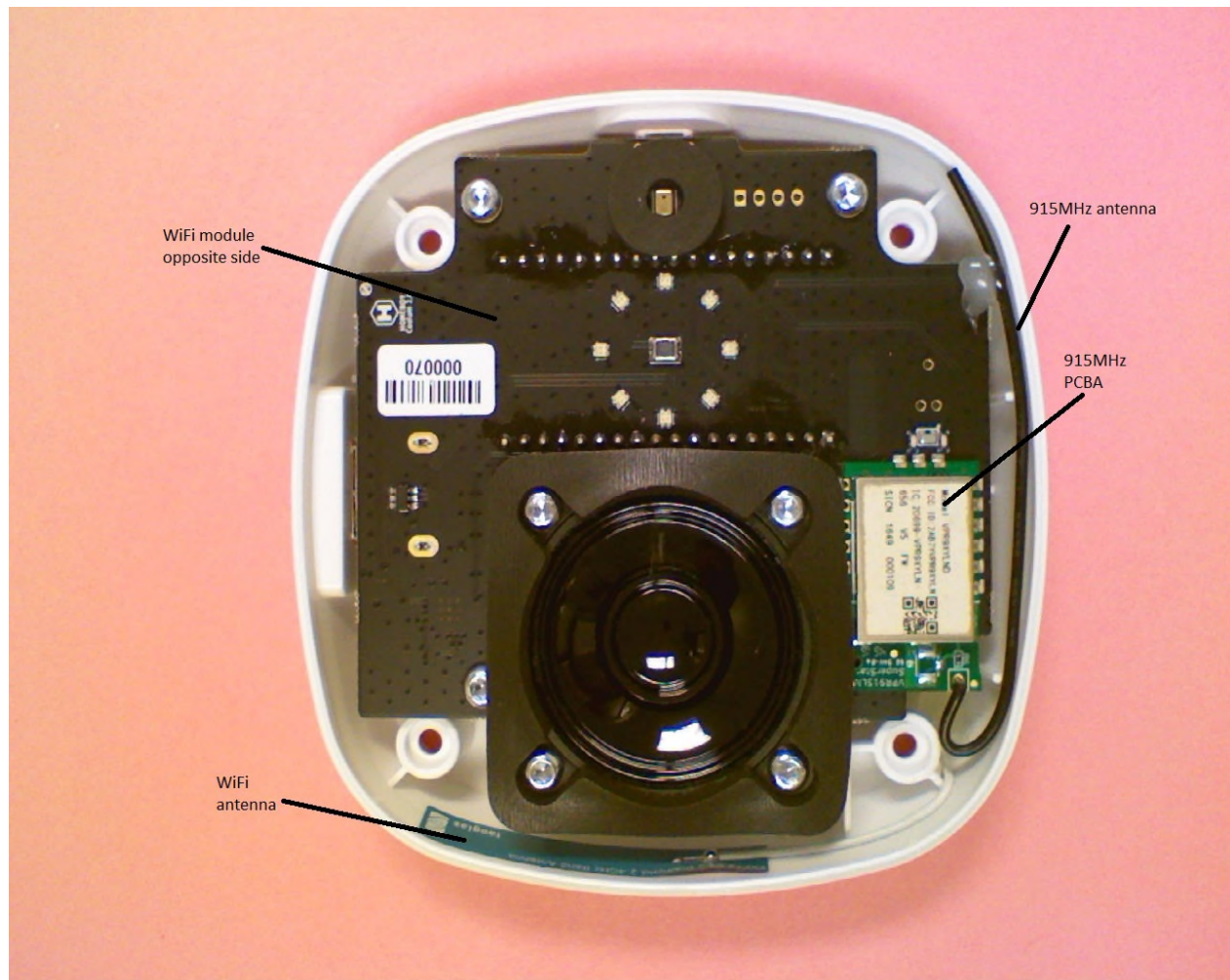
Figure 8: Module in Host
