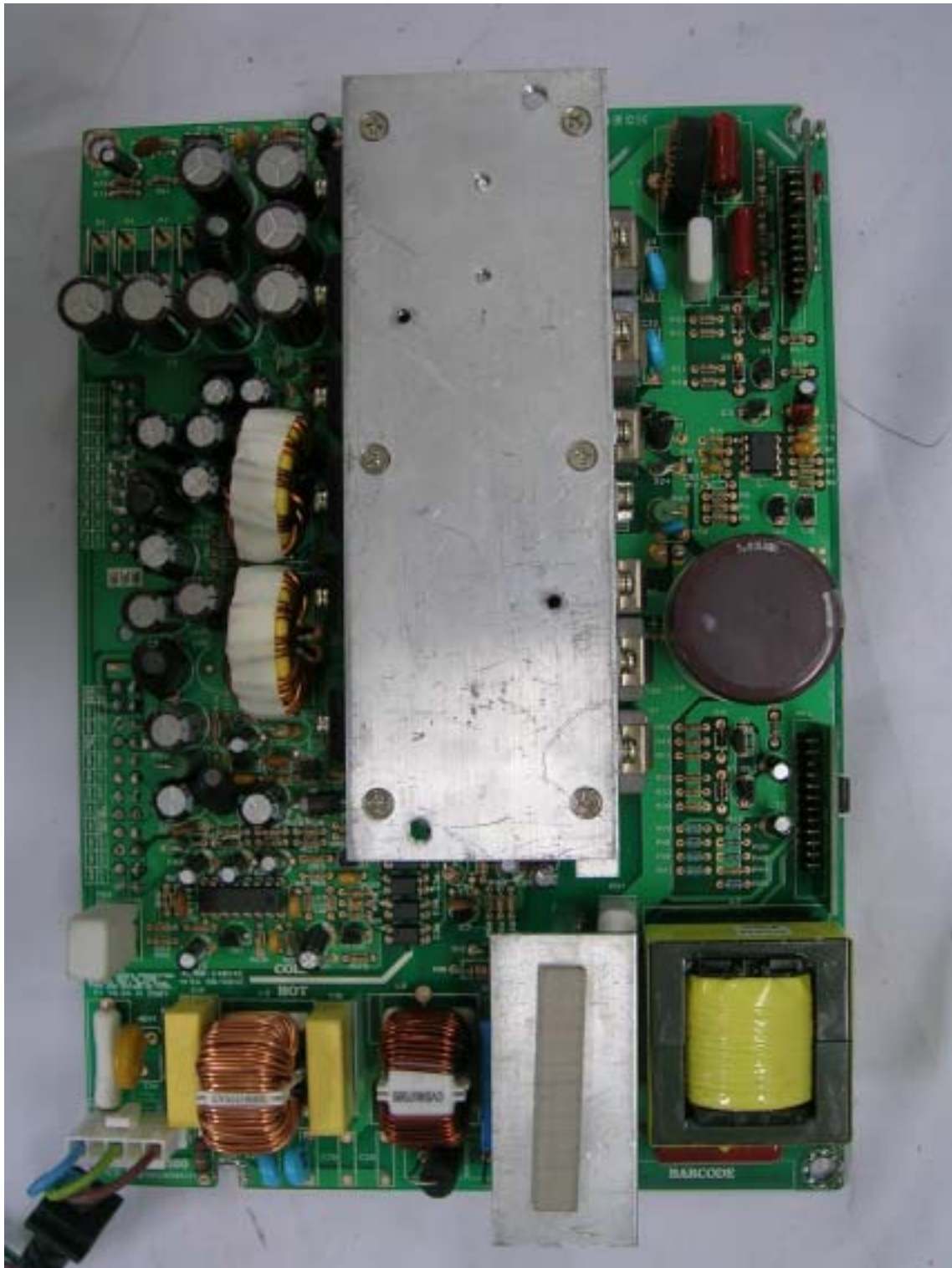
<FRONT VIEW OF SMPS BOARD>
