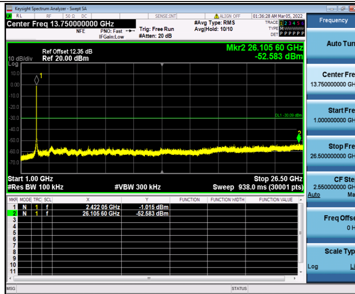
11AC40SISO_Ant2_2422_0~Reference
