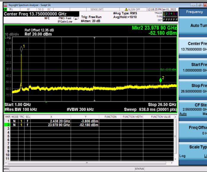
11N40SISO_Ant2_2437_0~Reference
