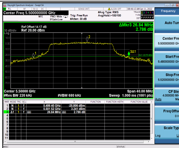
11AC20SISO_Ant2_5500
