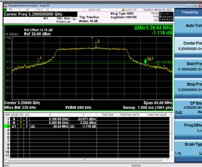
11AC20SISO_Ant2_5200
