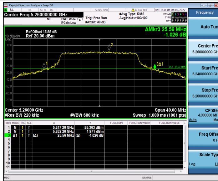
11AC20SISO_Ant2_5260
