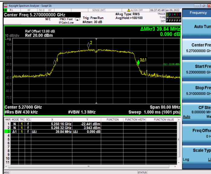
11AC40SISO_Ant2_5270
