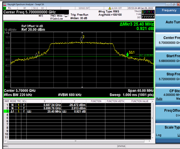
11AC20SISO_Ant2_5700
