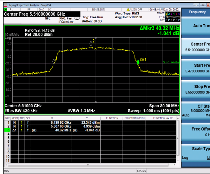
11AC40SISO_Ant2_5510
