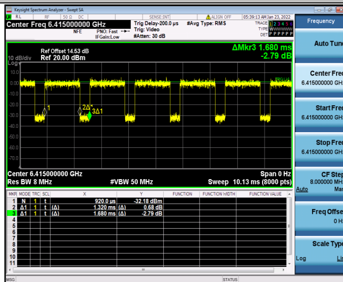
11AC20SISO_Ant1_6415
