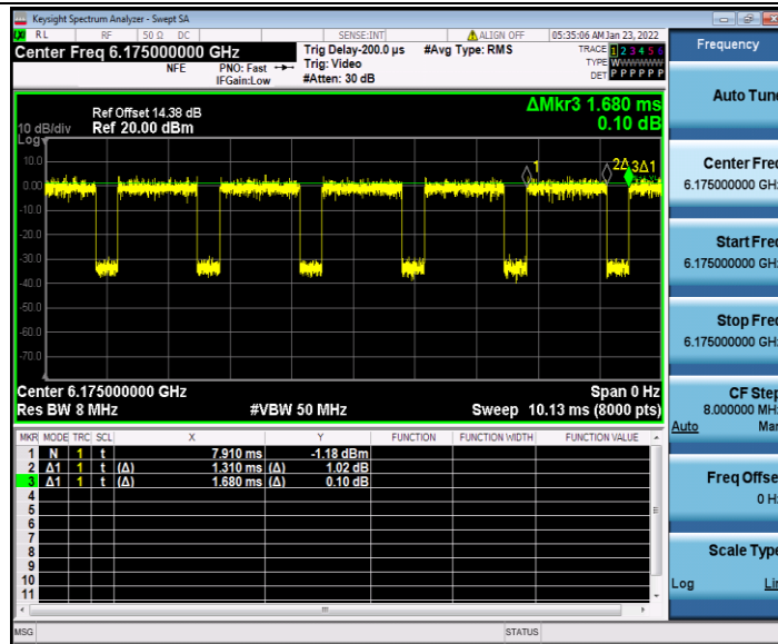
11AC20SISO_Ant2_6175
