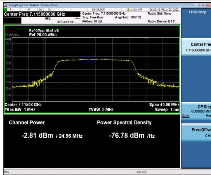
11AC20SISO_Ant2_7115
