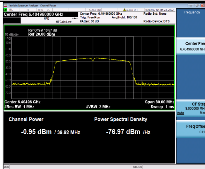
11AC40SISO_Ant2_6405
