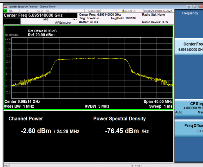
11AC20SISO_Ant1_6695
