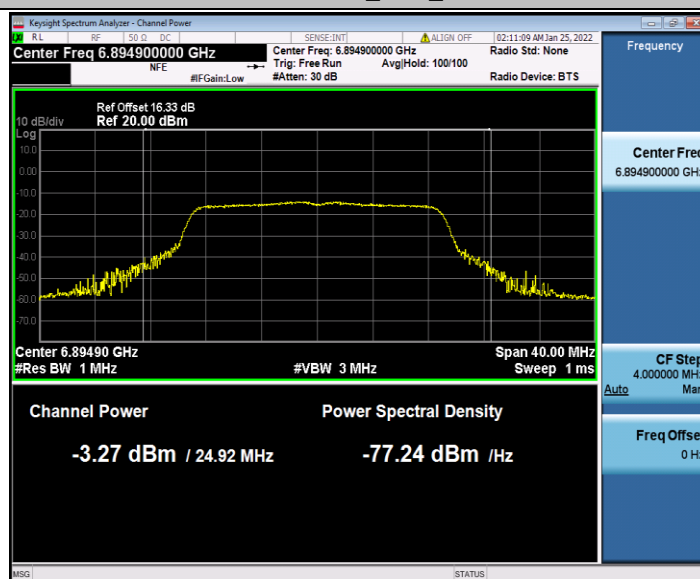
11AC20SISO_Ant2_6895
