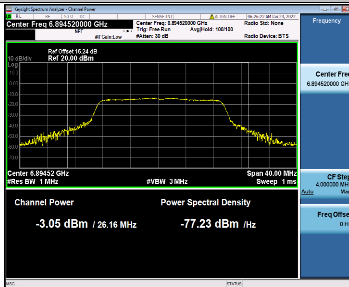
11AC20SISO_Ant2_6895
