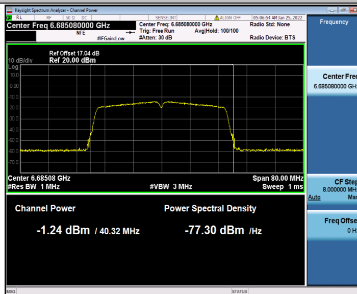
11AC40SISO_Ant2_6685
