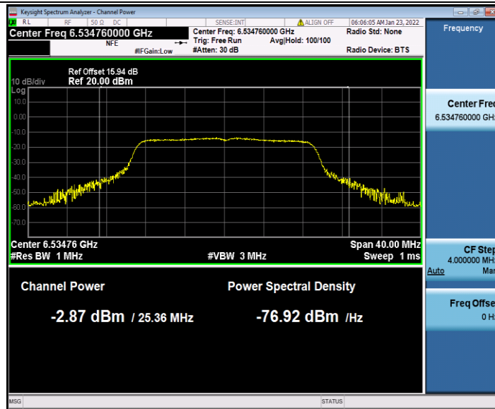
11AC20SISO_Ant2_6535
