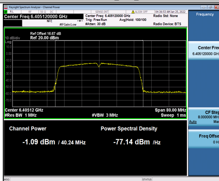
11AC40SISO_Ant2_6405
