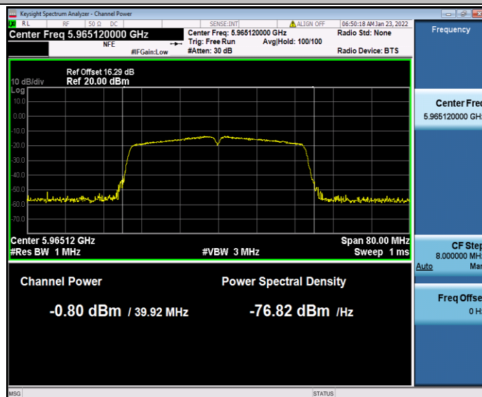
11AC40SISO_Ant1_5965
