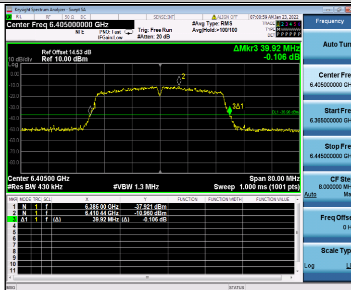
11AC40SISO_Ant2_6405
