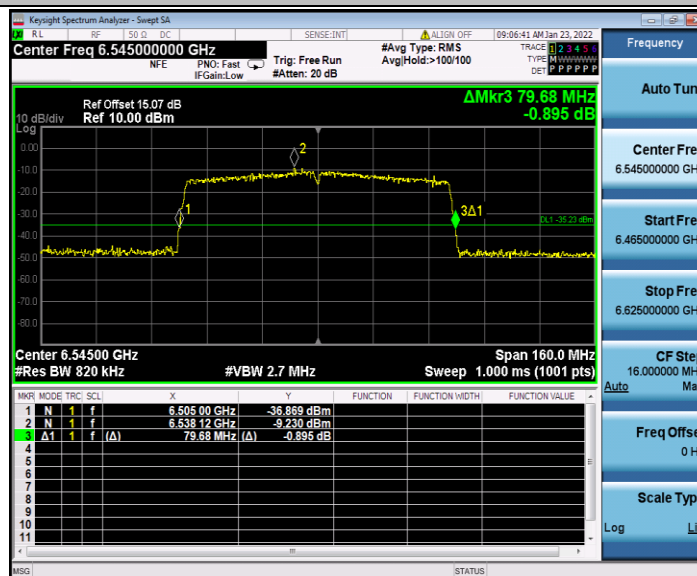
11AC80SISO_Ant2_6545
