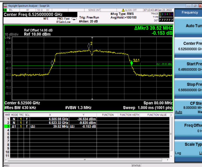
11AC40SISO_Ant1_6525
