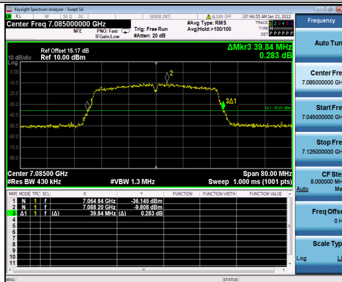
11AC40SISO_Ant2_7085
