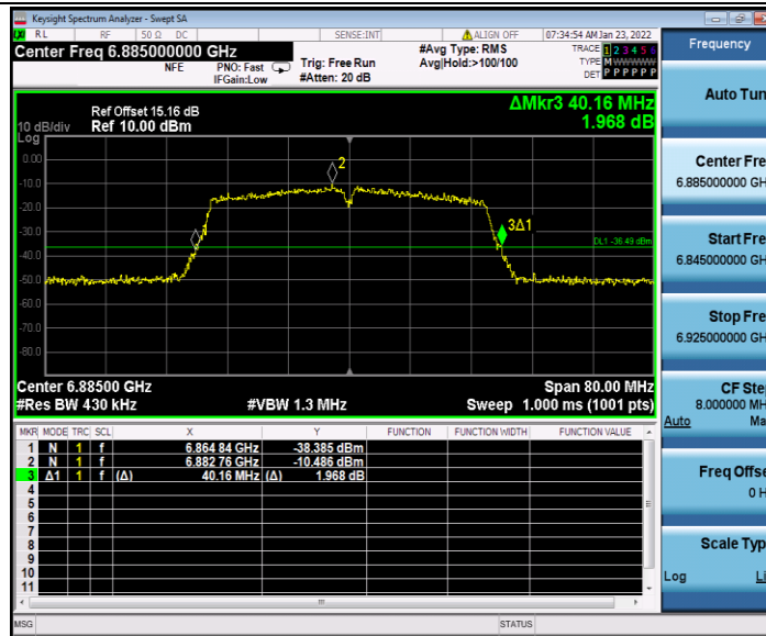
11AC40SISO_Ant2_6885
