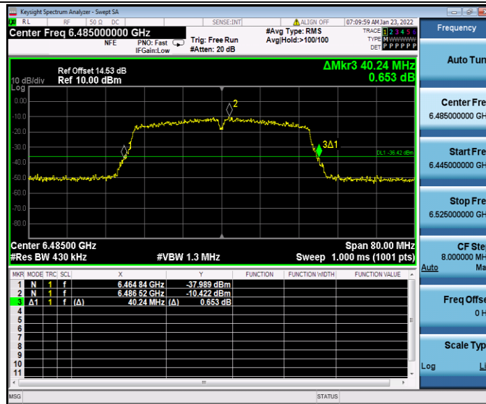
11AC40SISO_Ant2_6485
