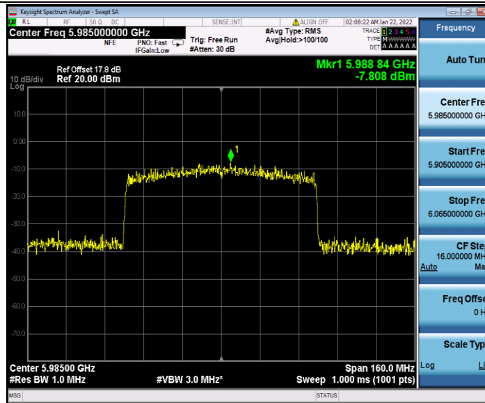
11AX80SISO_Ant2_5985
