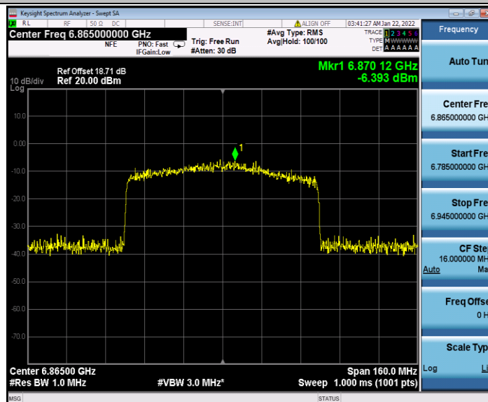
11AX80SISO_Ant2_6865
