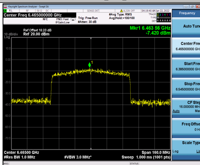
11AX80SISO_Ant2_6465
