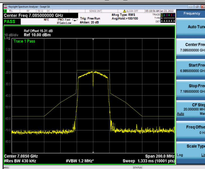
11N40SISO_Ant2_7085
