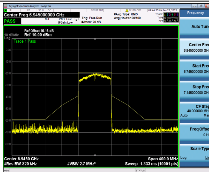
11AC80SISO_Ant2_6945
