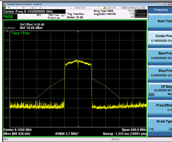
11AC80SISO_Ant2_6145
