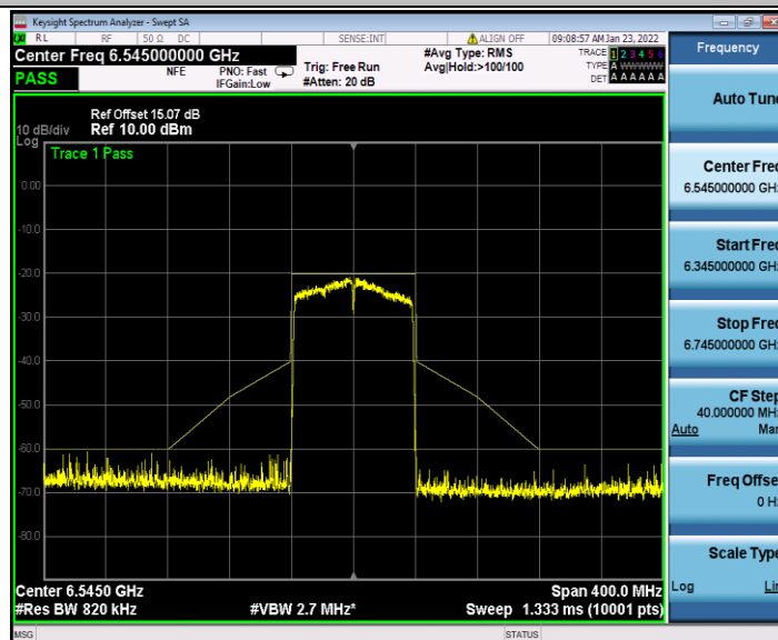
11AC80SISO_Ant2_6545
