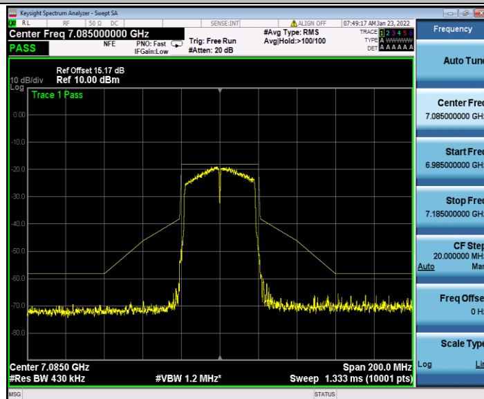
11AC40SISO_Ant2_7085
