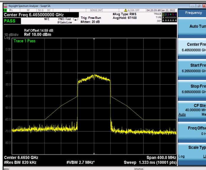
11AX80SISO_Ant2_6465
