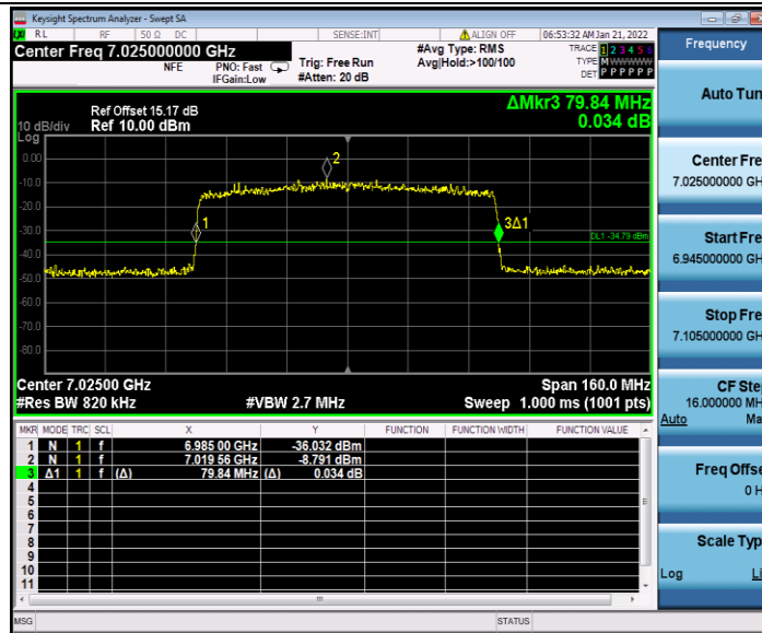
11AX80SISO_Ant2_7025
