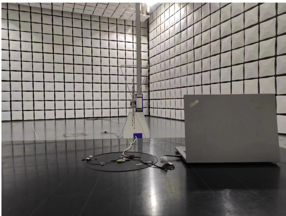
30MHz~1GHz
