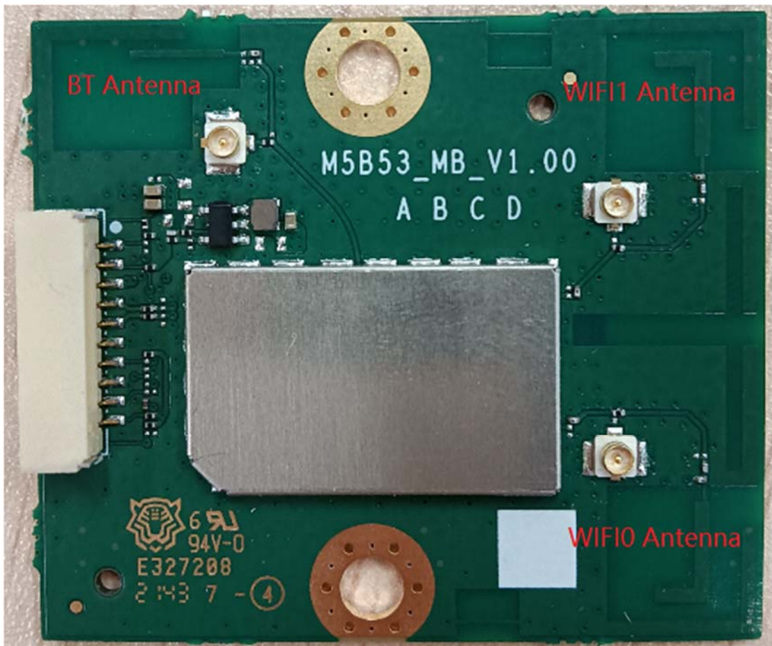
Antenna Location
