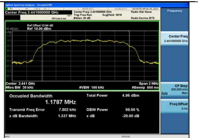
Test Mode: \pi/4 QPSK(2DH5) MHz
