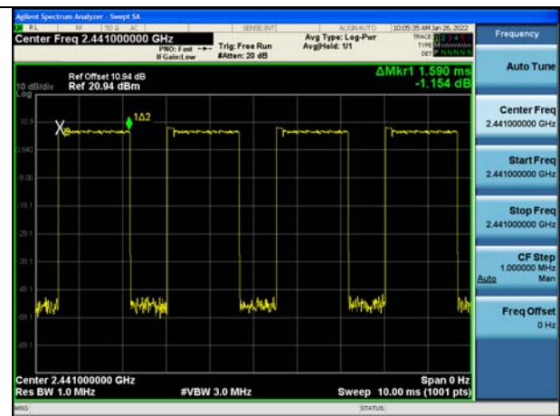
Test Mode: \pi/4 DQPSK(2DH5) 2441MHz
