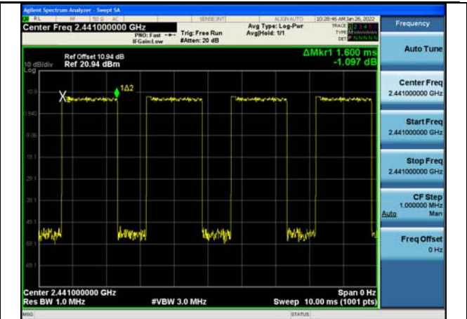
Test Mode:8DPSK(3DH5) 2441MHz
