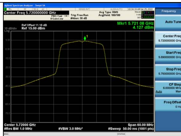
Test Mode:802.11ac VHT20 5720MHz Chain1 NII2C
