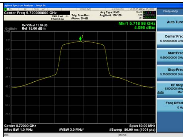
Test Mode:802.11n HT20 5720MHz Chain1 NII2C
