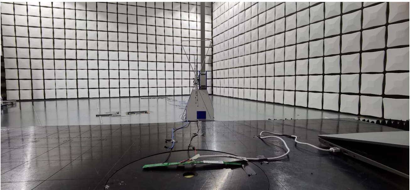
30MHz~1GHz
