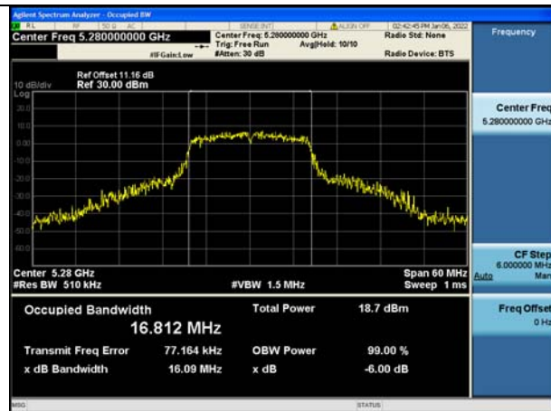
Test Mode:802.11a 5280MHz Chain0
