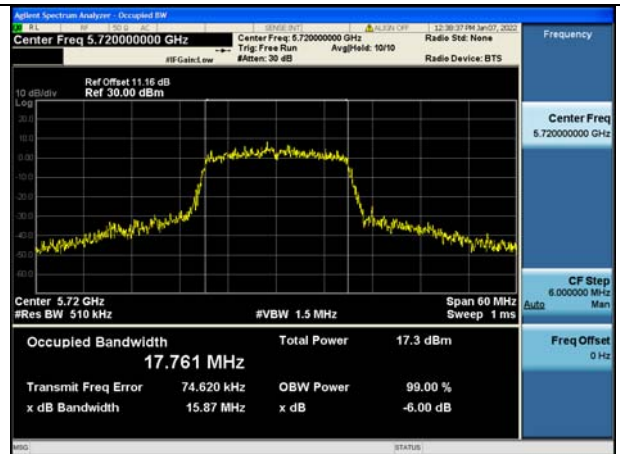
Test Mode:802.11ac VHT20 5720MHz Chain1 NII2C
