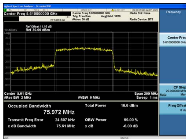
Test Mode:802.11ac VHT80 5610MHz Chain1
