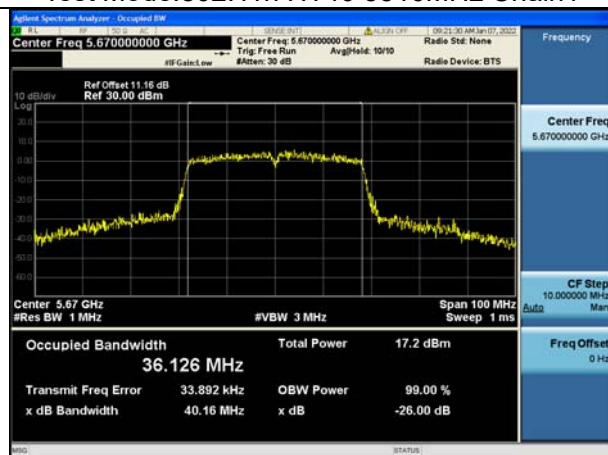
Test Mode:802.11n HT40 5670MHz Chain1
