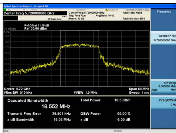
Test Mode:802.11a 5720MHz Chain1 NII2C
