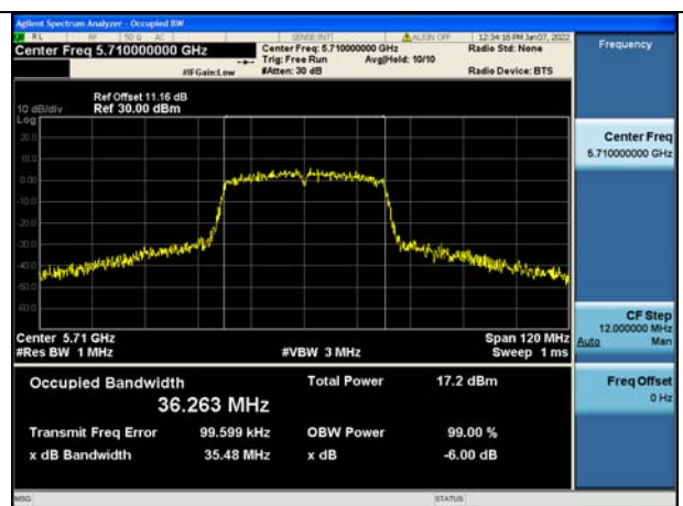
Test Mode:802.11n HT40 5710MHz Chain1 NII2C
