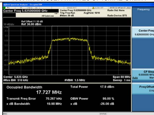
Test Mode:802.11n HT20 5825MHz Chain1
