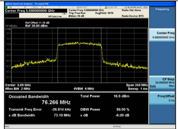
Test Mode:802.11ac VHT80 5690MHz Chain1 NII2C
