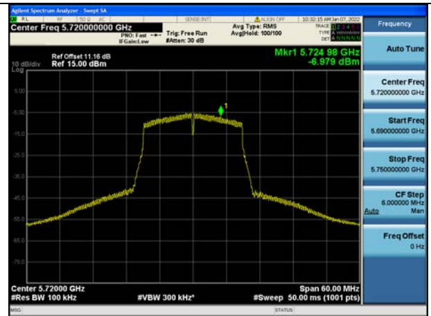
Test Mode:802.11n HT20 5720MHz Chain1 NII3
