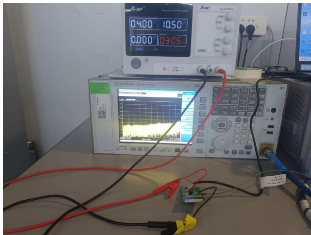
RF Conducted Test setup (BT/WIFI)
