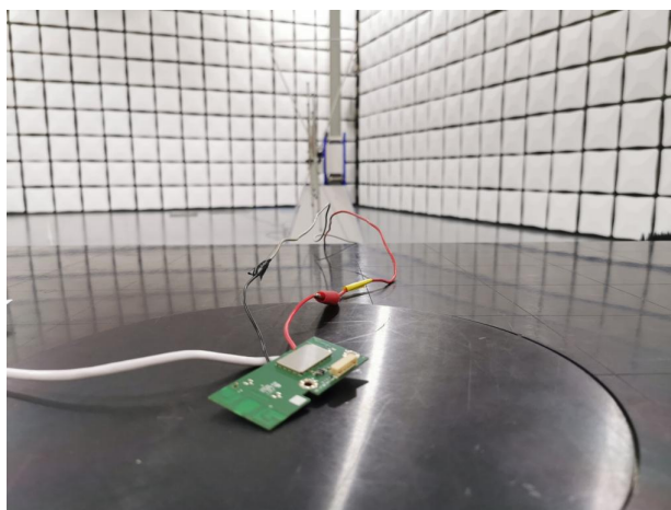
30MHz~1GHz
