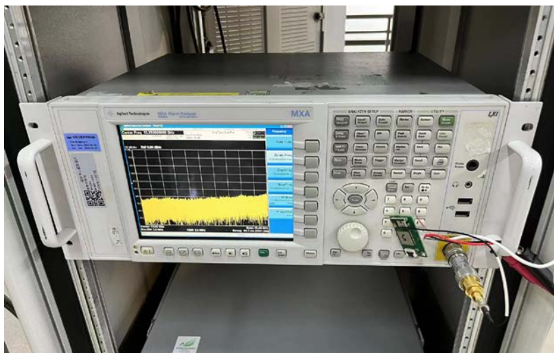
RF Conducted Test setup (WIFI)
