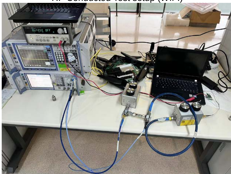
RF Conducted Test setup (DFS)
