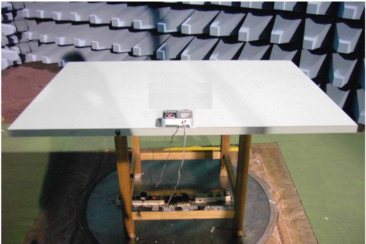
Rear View of the Test Configuration of X-axis
