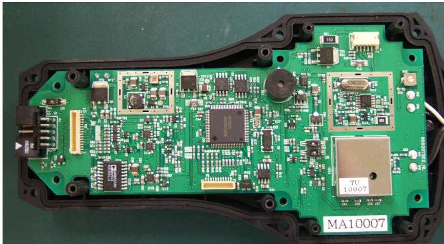
TOP View of MAIN PCB
