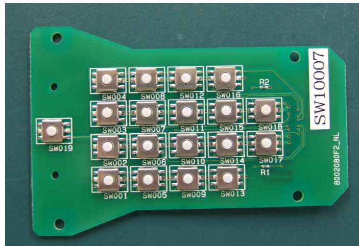
TOP View of SWITCH PCB
