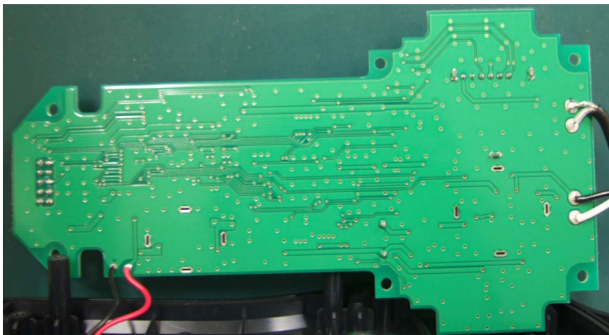
BOTTOM View of MAIN PCB
