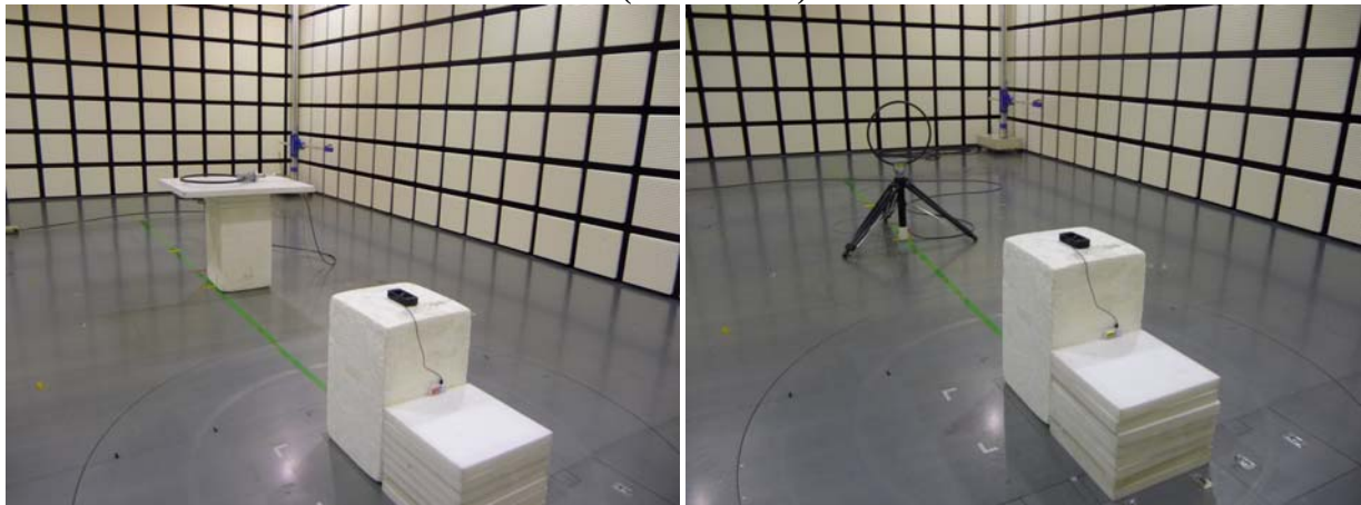
Rear (9kHz-30MHz)
