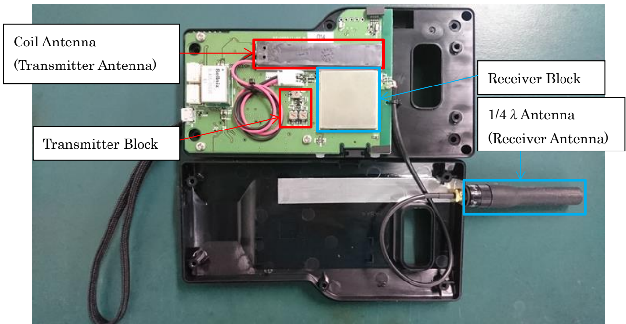
Wireless Block and Antenna Position
