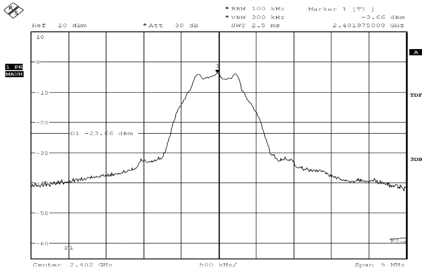
Diagram 1: 20dBc Reference
