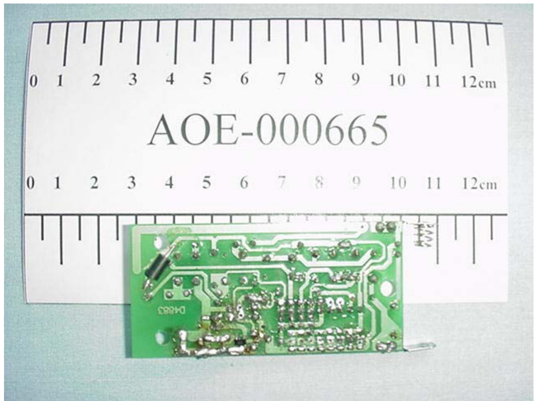
FIGURE 3 REMOTE DEER CALL (M/N: CY-01) MAIN BOARD (SOLDERED SIDE)
