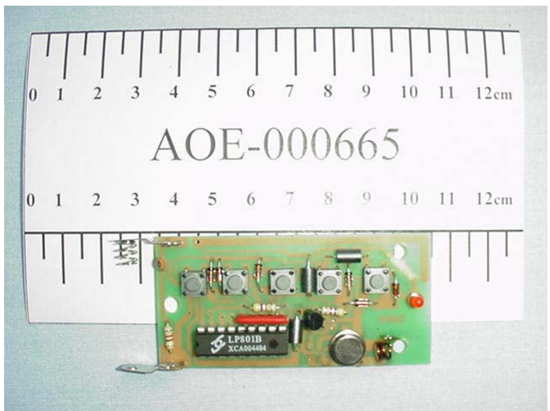
FIGURE 2 REMOTE DEER CALL (M/N: CY-01) MAIN BOARD (COMPONENT SIDE)
