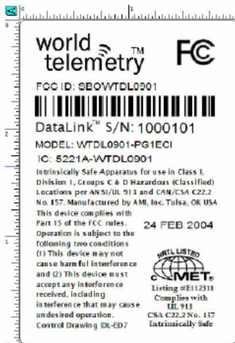
Front Label
