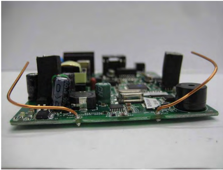
EUT Antenna, View #2 (Photo taken by CKC Laboratories)
