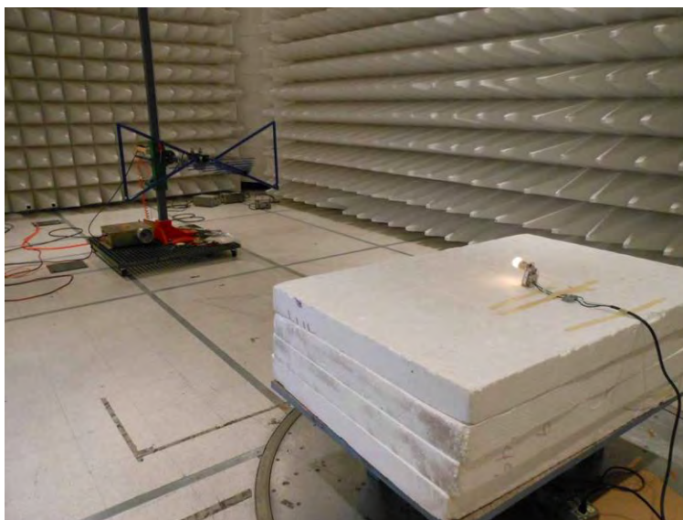
30MHz-1GHz
