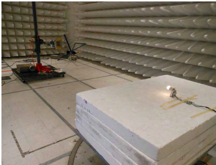
1-10GHz
