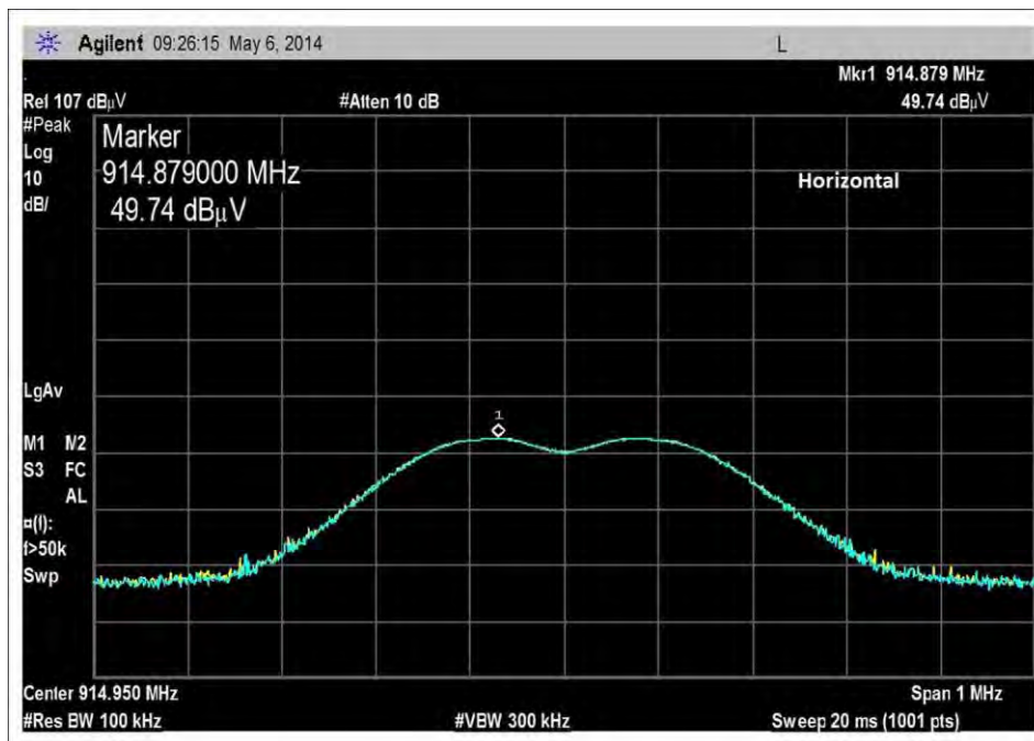
Horizontal Polarization
